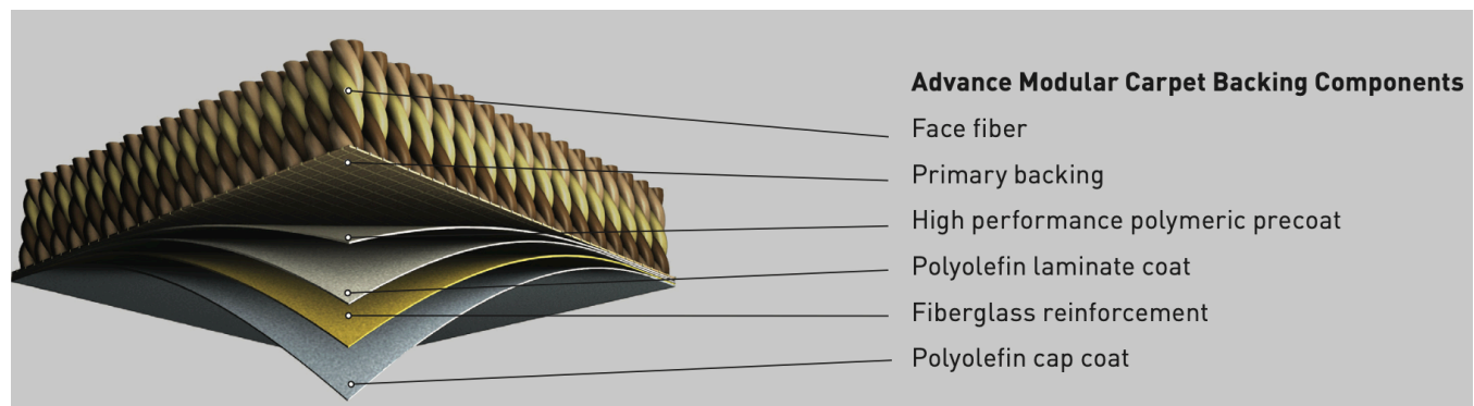
Figure 1: Product Construction
