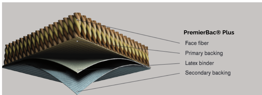
Figure 1: Product Construction
